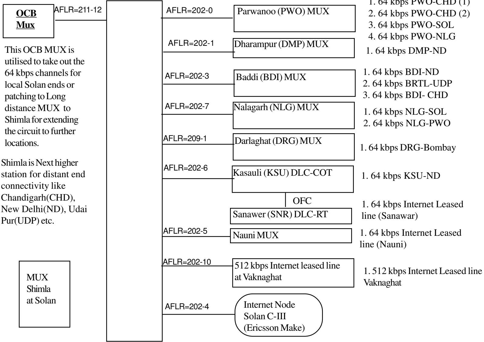
Fig 1 : SSA Solan Leased Line Network Diagram
